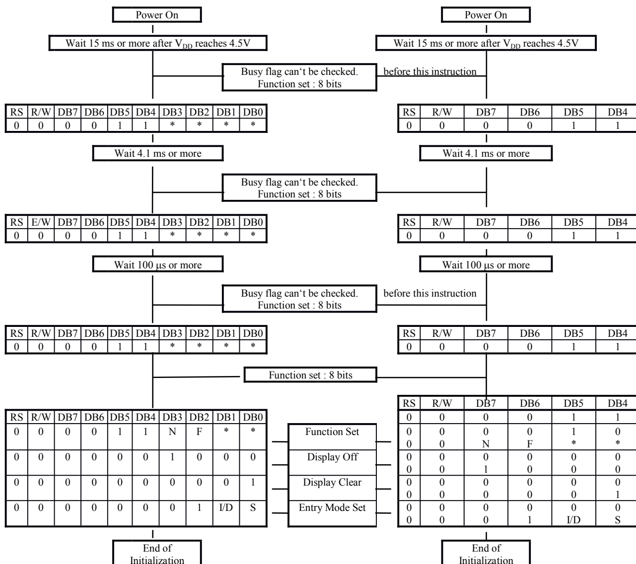
1) 8 Bit Interface
