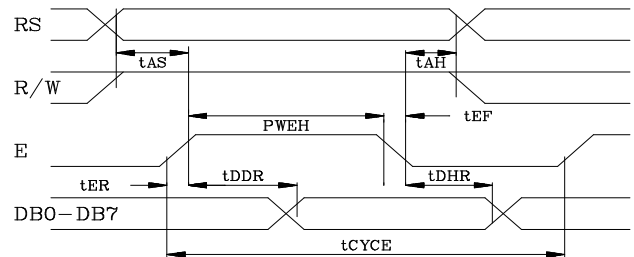
Read Operation
